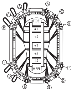
Bottom View of Moon Shoe®
